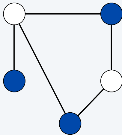
bipartite (2-colorable)
